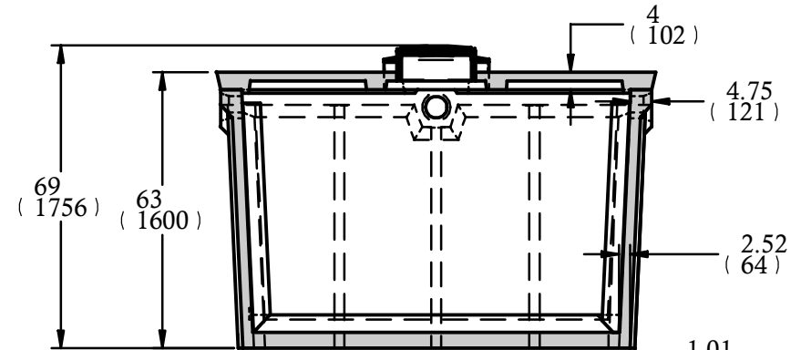
SECTION B-B in | mm |
