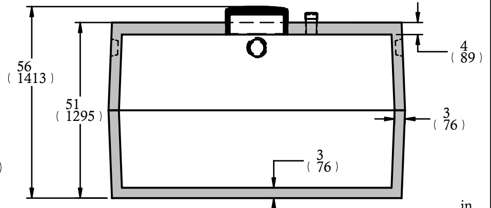
SECTION B-B
