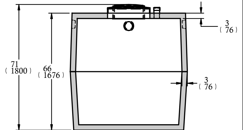
SECTION B-B
