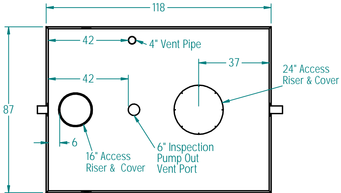
TANK LID PLAN VIEW
