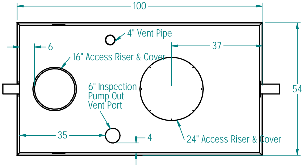
TANK LID PLAN VIEW
