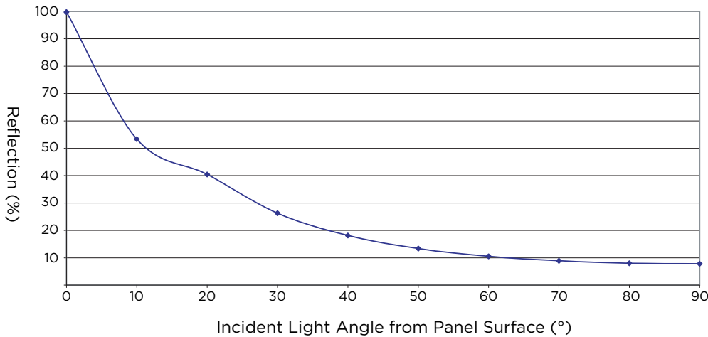
FIGURE 2 - REFLECTION OF ACRYLITE® SOUNDSTOP
